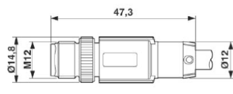
Assembled cable coupling
