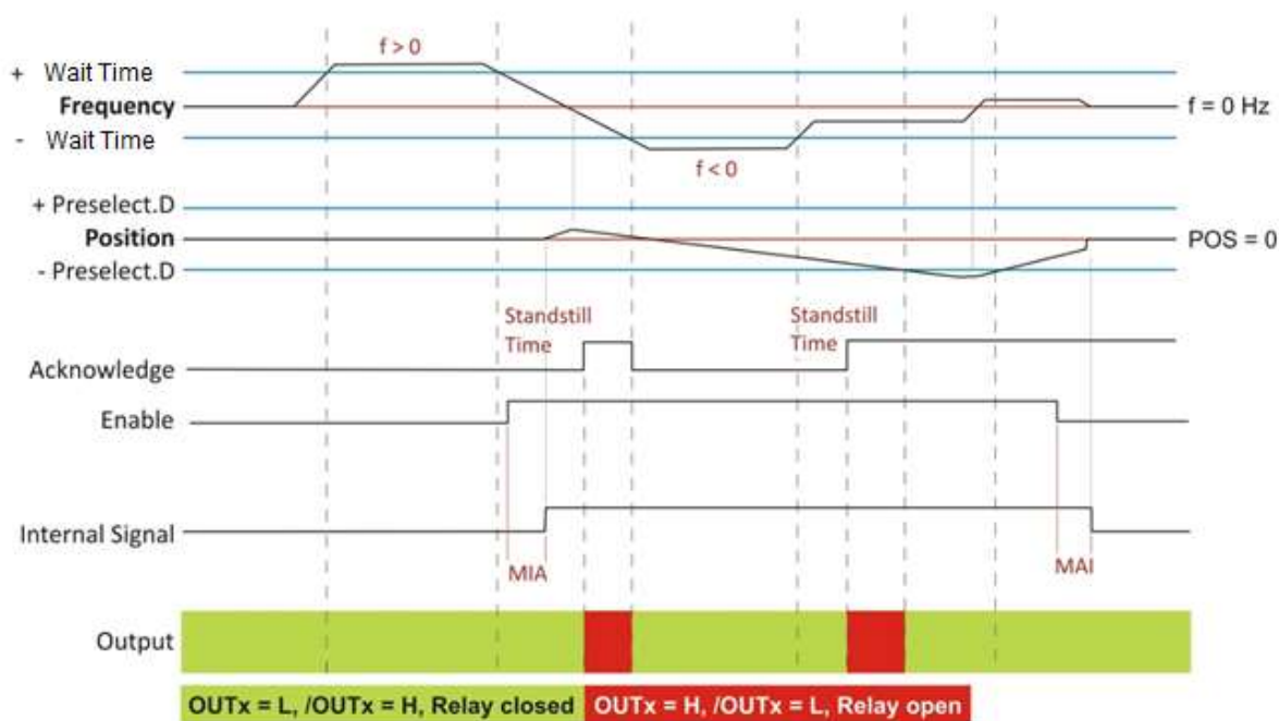
Standstill Monitor: with static high Enable Input
